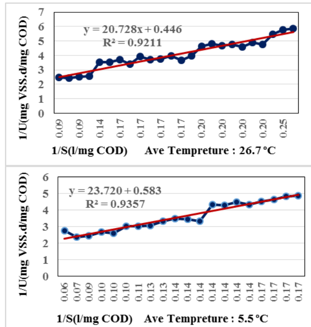
Figure 4. Monod model
