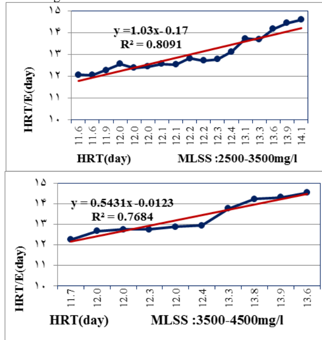
Figure 2. Grau second-order substrate removal model
