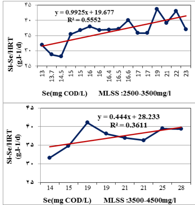
Figure 1. First-order substrate removal model
