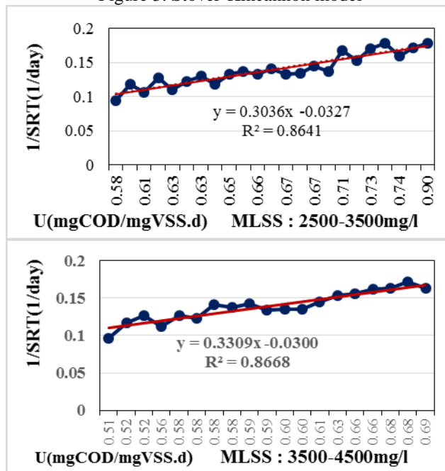
Figure 3. Stover-Kincannon model
