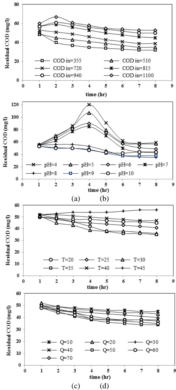
Figure 1. (a) Variation of residual COD concentration at different influent COD concentrations (pH=8, T=30 °C, Q= 80 l/min). (b) Variation of residual COD concentration at different pH (T= 30 °C, COD in = 600 mg/l, Q= 80 l/min). (c) Variation of residual COD concentration at different temperatures (pH=8, COD in =600 mg/l, Q= 80 l/min). (d) Variation of residual COD concentration at different airflow rates (pH=8, T=30 °C, COD in = 600 mg/l).
